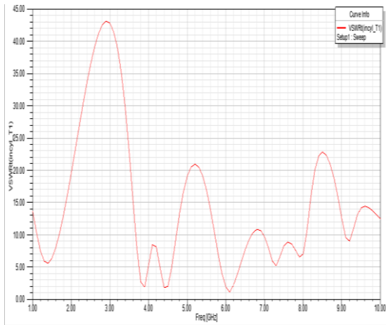
Figure 7: VSWR Vs. Frequency for Proposed Antenna One of important parameter is smith chart. By using smith chart one can have obtained reflection coefficient, maxima location, impedance matching and many other things. Figure 8 shows smith chart of proposed antenna.
