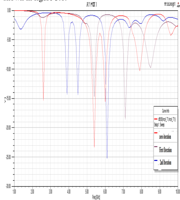
Figure 5: Return Loss Vs. Frequency for Different Fractal Iterations of T-shaped FMPA
