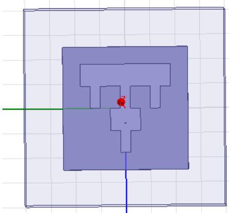
Figure 2: Antenna with DGS using Different Substrate
