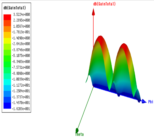
Figure 6(c): Radiation Pattern of T-shaped FMPA at 6.1 GHz
