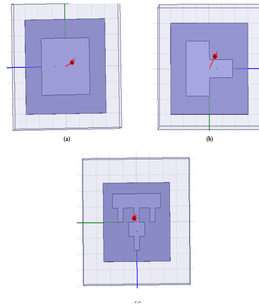
Fig 1: T- Shaped FMPA (a) 0 th Iteration, (b) 1 st Iteration and (c) 2 nd Iteration
