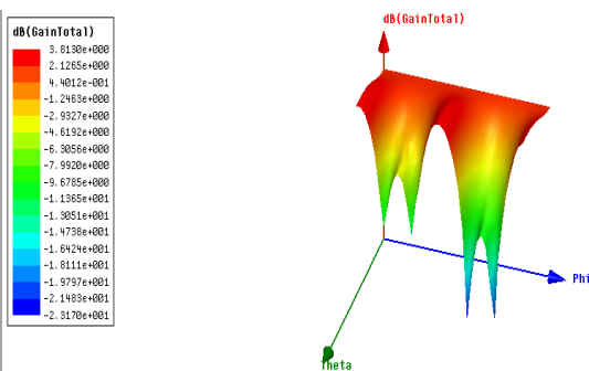
Figure 6(b): Radiation Pattern of T-shaped FMPA at 4.5 GHz
