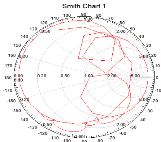
Figure 8: Smith Chart of Proposed Antenna
