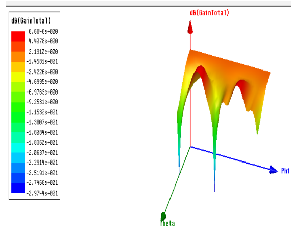
Figure 6(c): Radiation Pattern of T-shaped FMPA at 6.1 GHz
