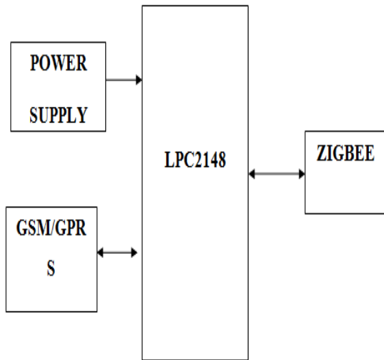
Fig 3. Wireless Information Unit
