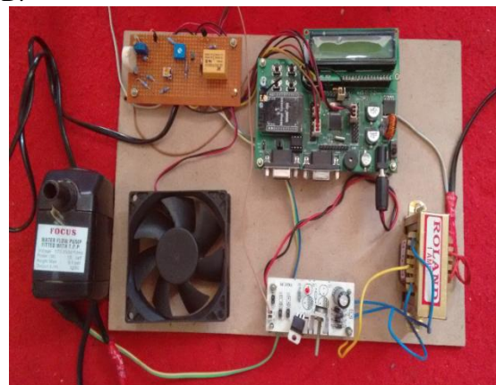
Fig 2. Transmission Section
