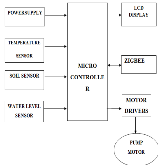
Fig 1. Wireless Sensor Unit
