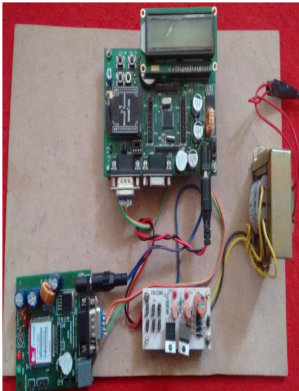
Fig 4. Receiver Section
